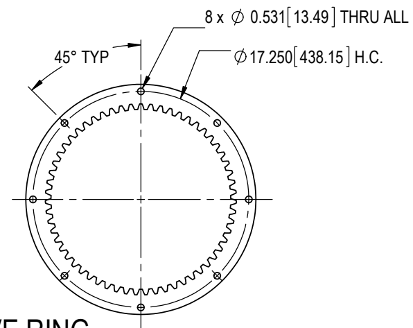
DRIVE RING
